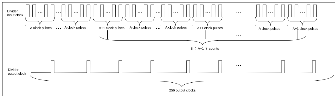
Figure 85: LED_PWM Divider
