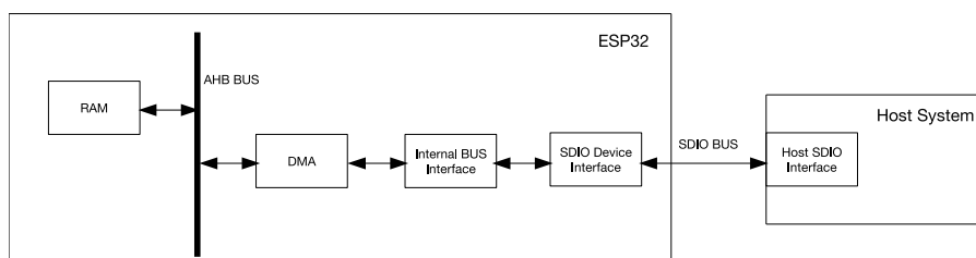
Figure 20: SDIO Slave Block Diagram
