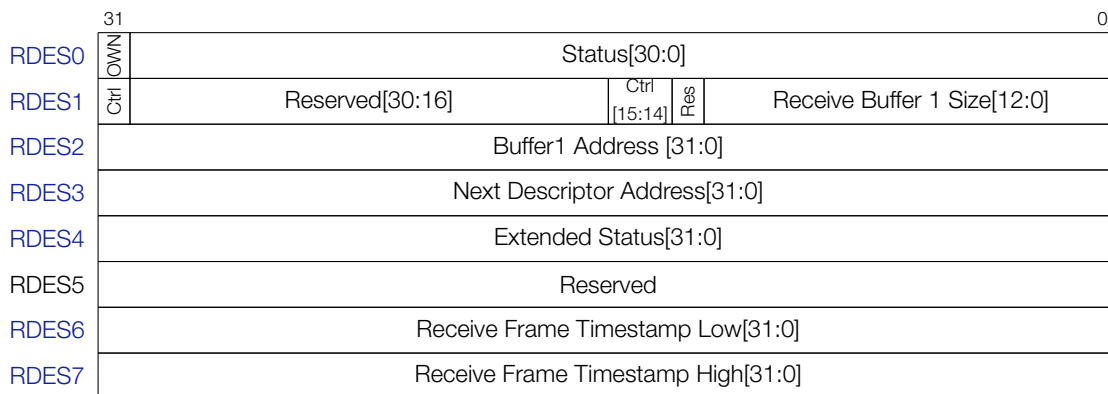
Figure 46: Receive Descriptor
