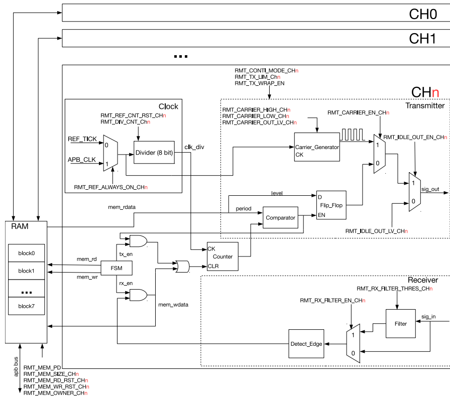
Figure 88: RMT Architecture
