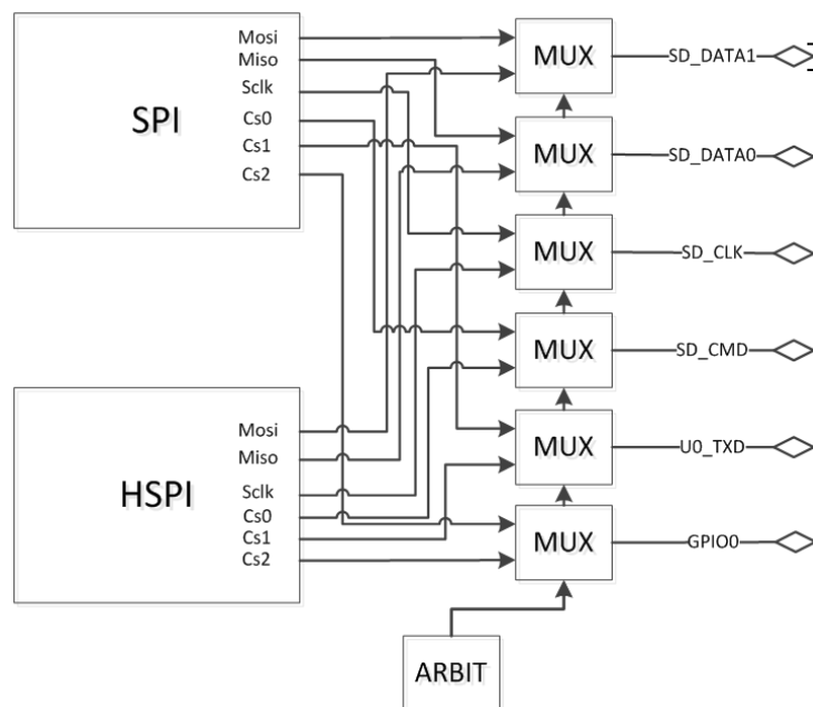
Figure 5-1. SPI Overlap Block Diagram
