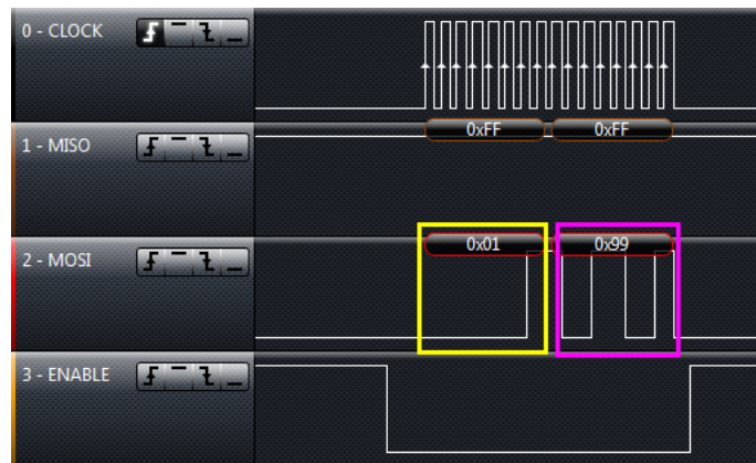
Figure 4-8. Waveform Graph 4
