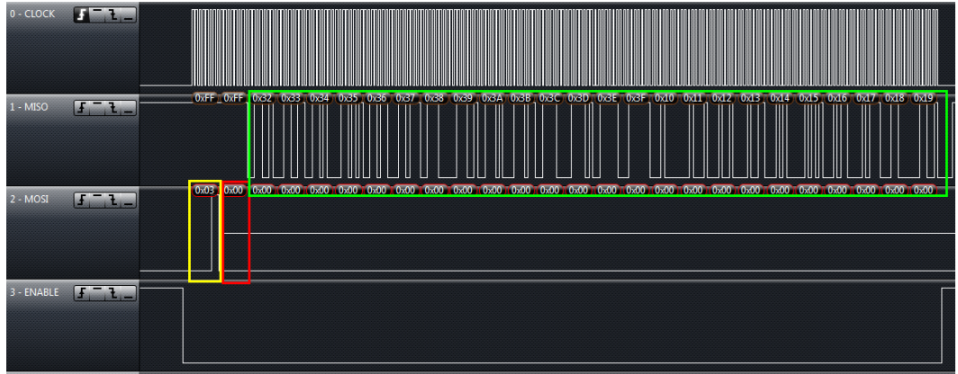
Figure 4-6. Waveform Graph 2
