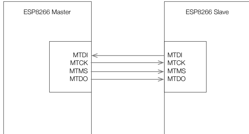
Figure 4-3. Test Demo Hardware Connection
