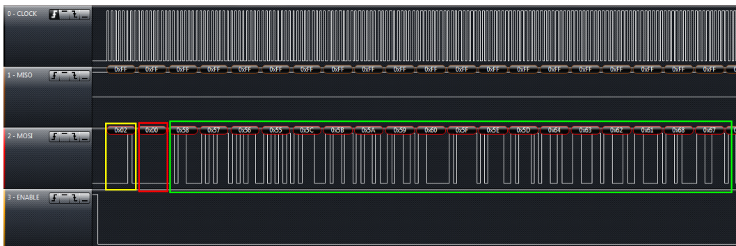
Figure 4-5. Waveform Graph 1
