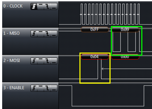
Figure 4-7. Waveform Graph 3
